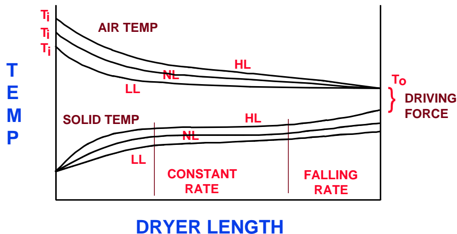
FIGURE 1 - DRIVING FORCE FOR DRYING PROBLEMS WITH USING EXHAUST TEMPERATURE CONTROL
